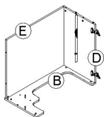
Cabinet Assembly
